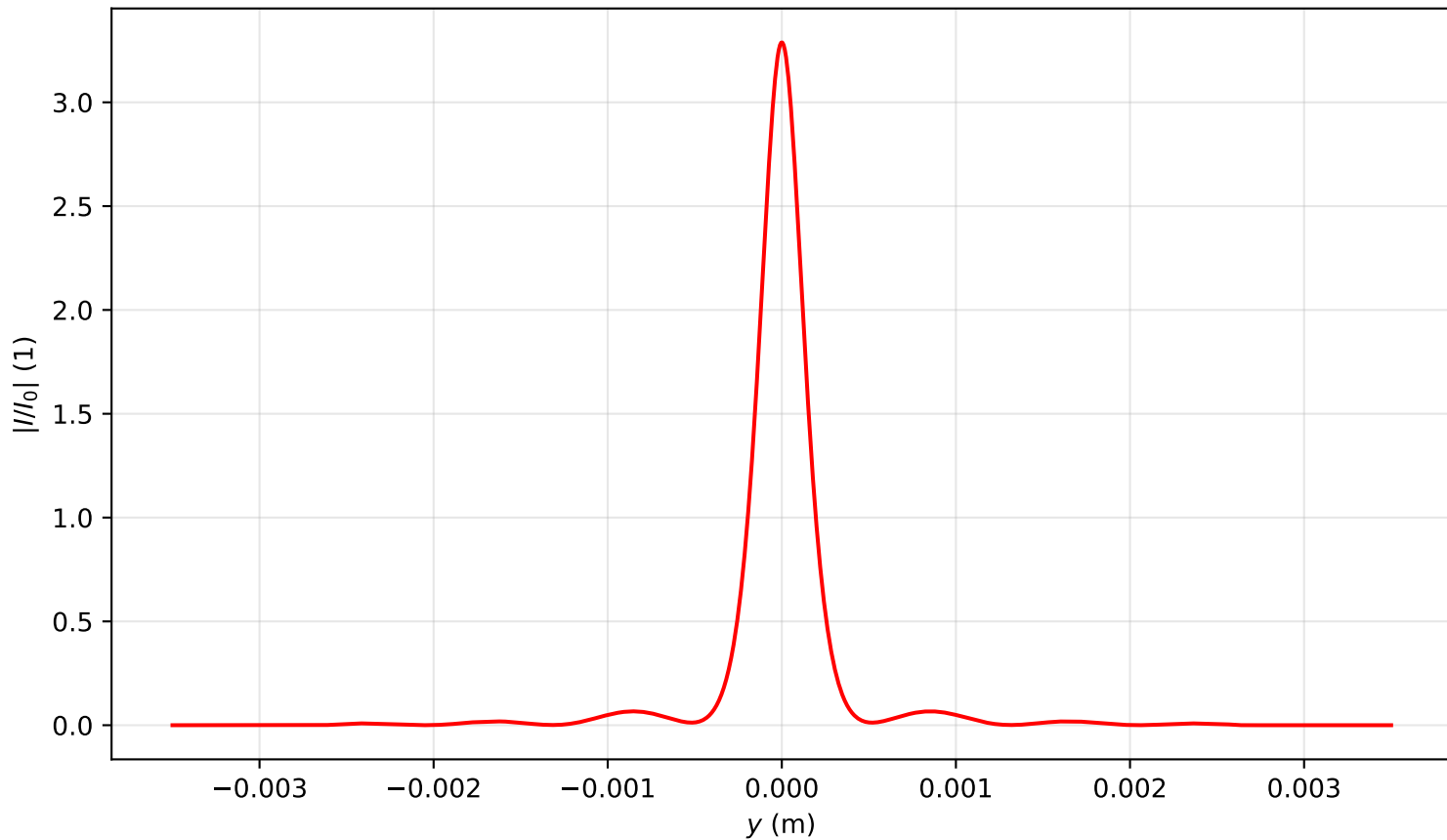
Intensity profile I(x = 0, y, z = 0.637)/I_0 , \text{Pin}=1.0\text{Pcr} , artificial time
